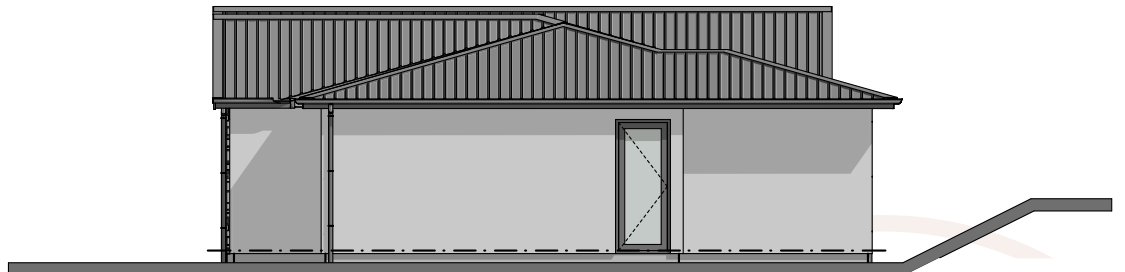
4 Waianiwa Place South Elevation Not To Scale
